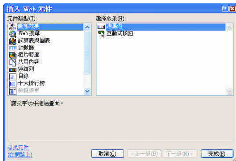
插入跑馬燈
